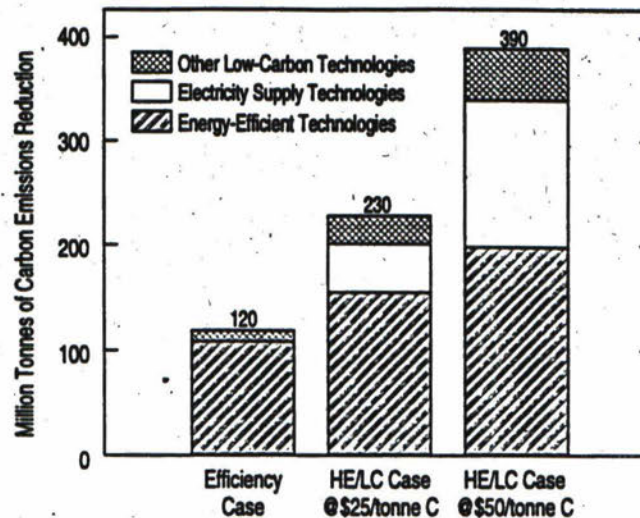
Figure 1.2 Reductions in Carbon Emissions from Each Scenario
