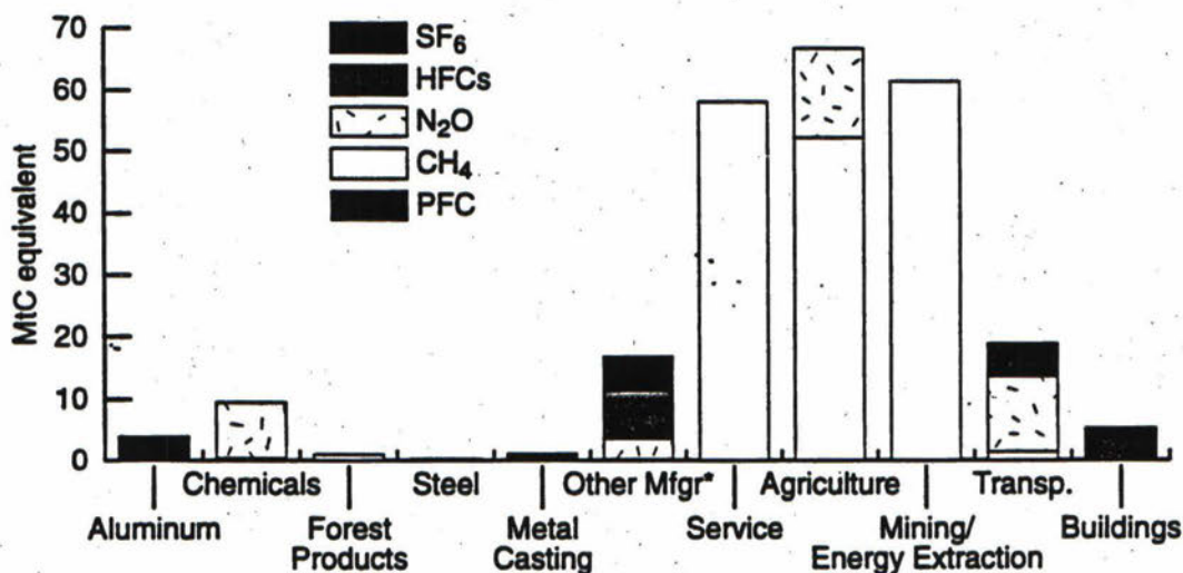
Figure 2.2 Non- \text{CO}_2 Greenhouse Gas Emissions by End-Use Sector and Industry
