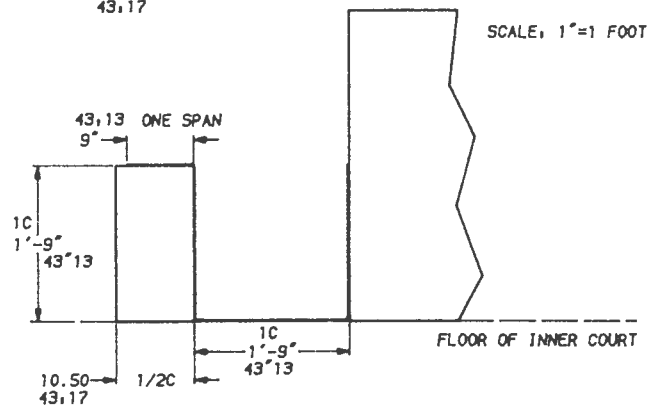
GUTTER DETAIL SECTION "A-A" 43.17
