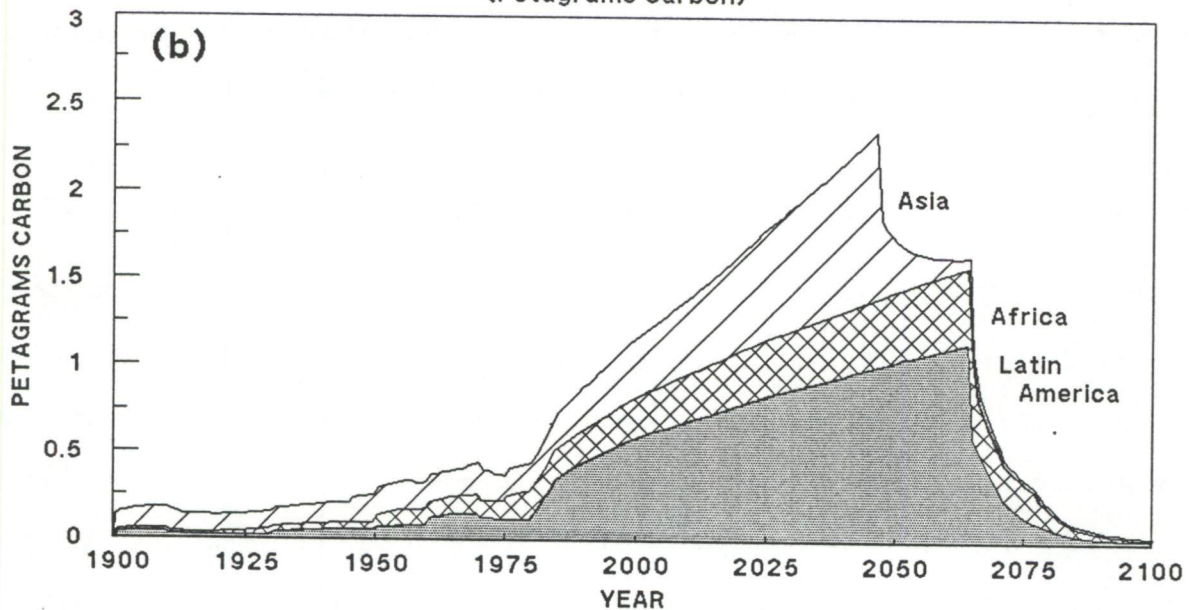
Figure 17. (a) Annual emissions of CO 2 from deforestation in units of carbon, based on the low estimate of initial biomass. The lowest curve (the dashed and dotted line) is assumed in both the SCWP and RCWP scenarios and indicates net uptake of CO 2 due to reforestation after 2000. (b) Regional detail for the SCW scenario. Sharp declines in emissions follow the exhaustion of forests in Asia, Africa, and Latin America.
