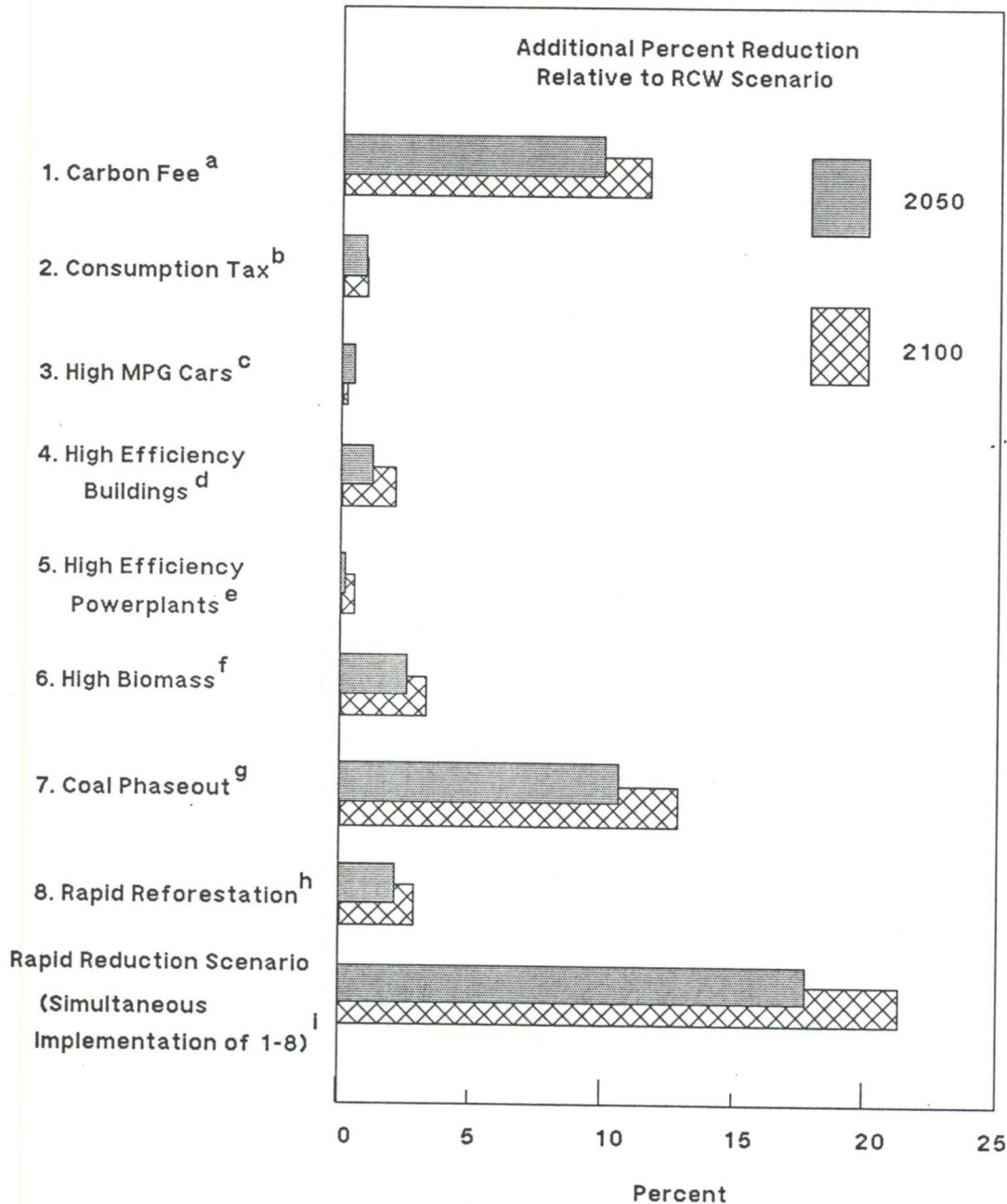
Figure 9. The impact of additional measures applied to the RCWP scenario expressed as percent change relative to the equilibrium warming commitment in the RCW scenario. The simultaneous implementation of all the measures in combination with the measures in the RCWP scenarios represents the Rapid Reduction scenario.
