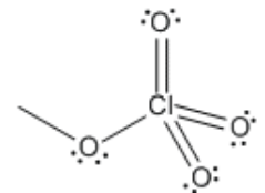
Perchlorate
