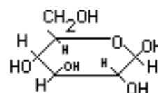
Beta Glucose
