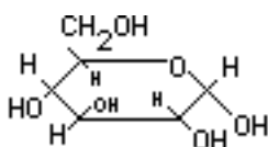
Alpha Glucose
