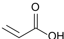
Acrylic Acid
