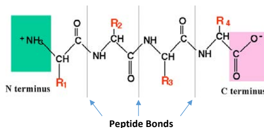
Polypeptide Structure
