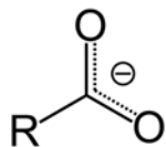
Carboxylate Ion
