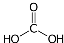
Carbonic Acid
