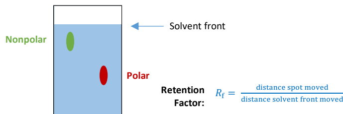
Thin-Layer Chromatography
